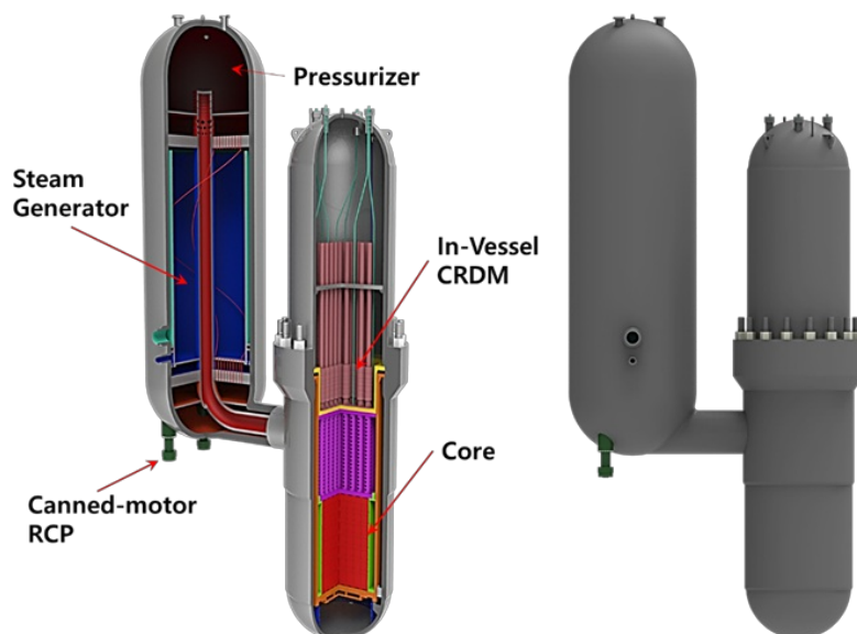
Figure 4. RCS configuration and cross sectional view of BANDI.
