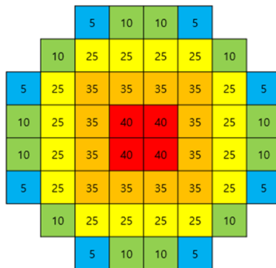
Figure 5. BANDI reactor core with burnable poison.
