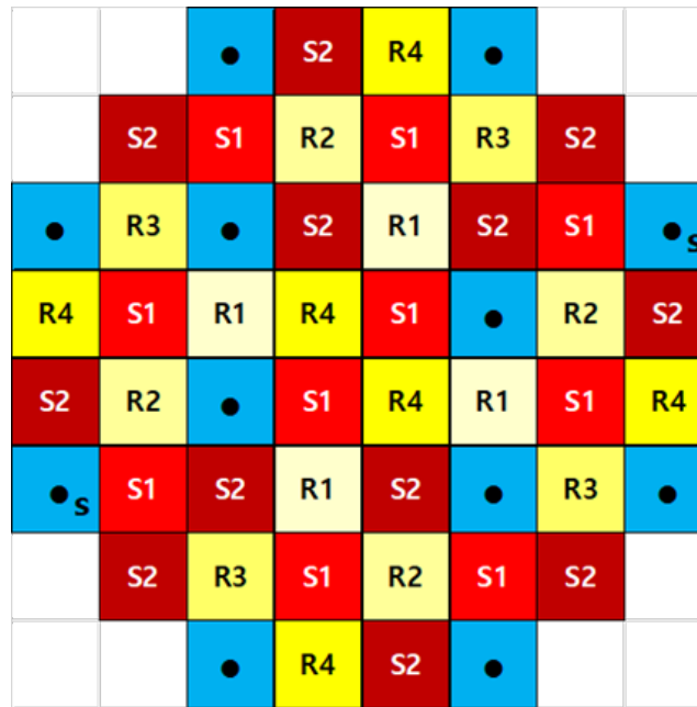
Figure 6. BANDI reactor control rod arrangement.
