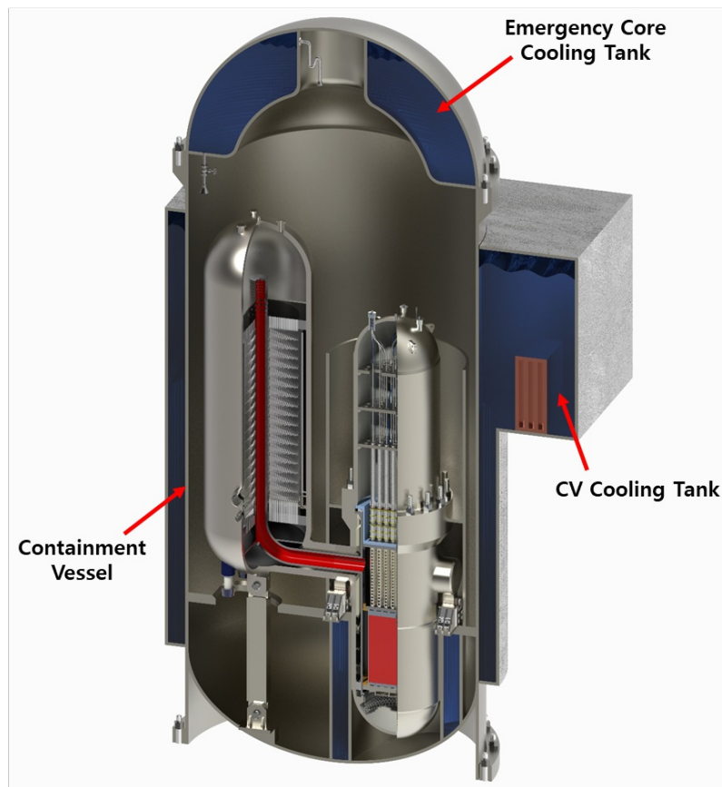
Figure 1. BANDI reactor coolant system and safety systems configuration.
