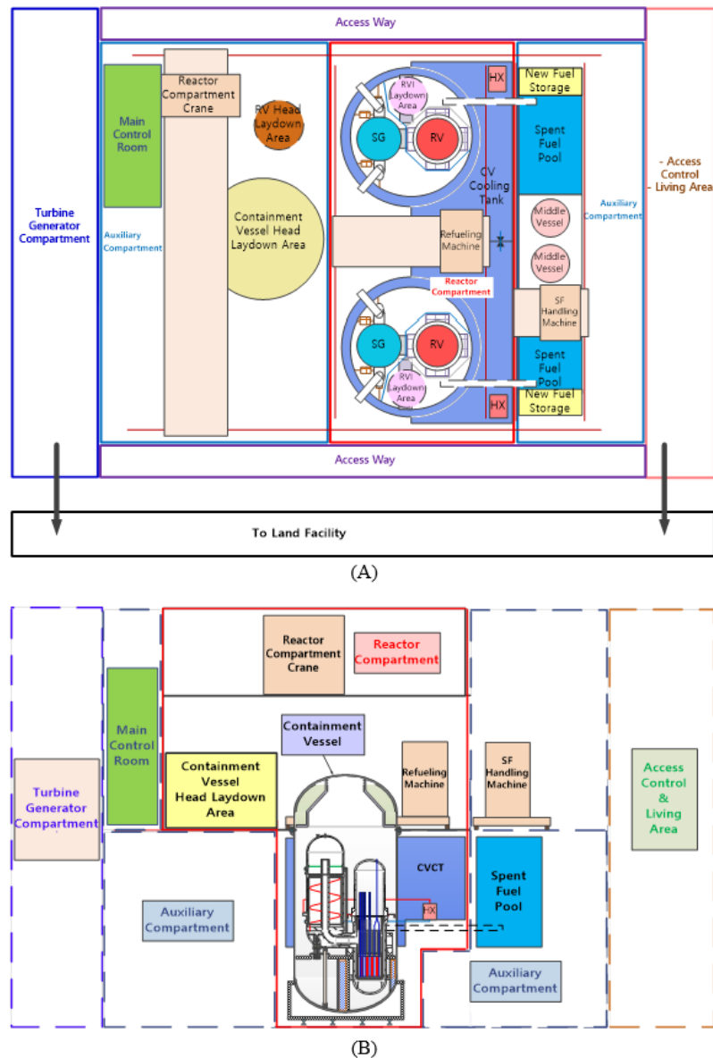
Figure 3. BANDI Floating Nuclear Power Plant: (A) Plane view and (B) Section view.
