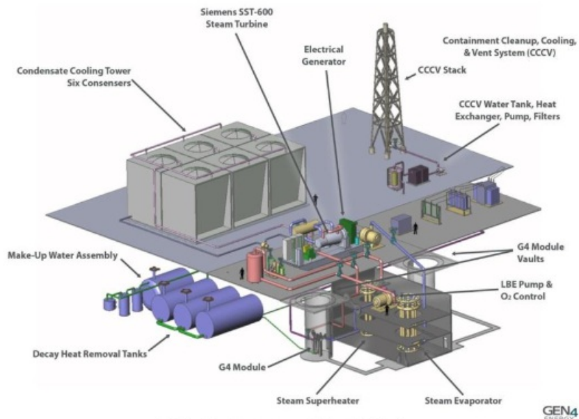
Figure 1. Description of G4M reactor
