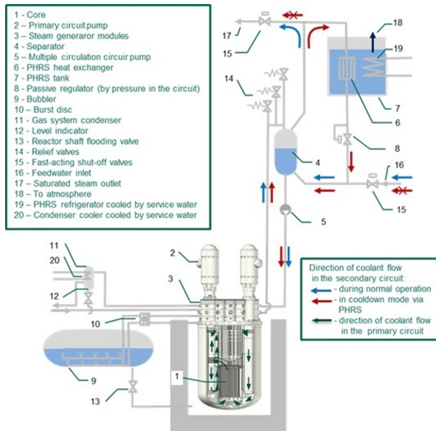
Figure 3. The basic hydraulic diagram of the NSSS SVBR-100.
