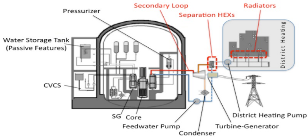
Figure 1. Plant layout
