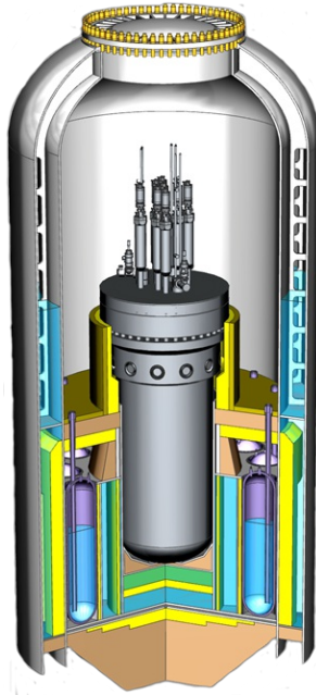
Figure 1. ABV-6E design concept
