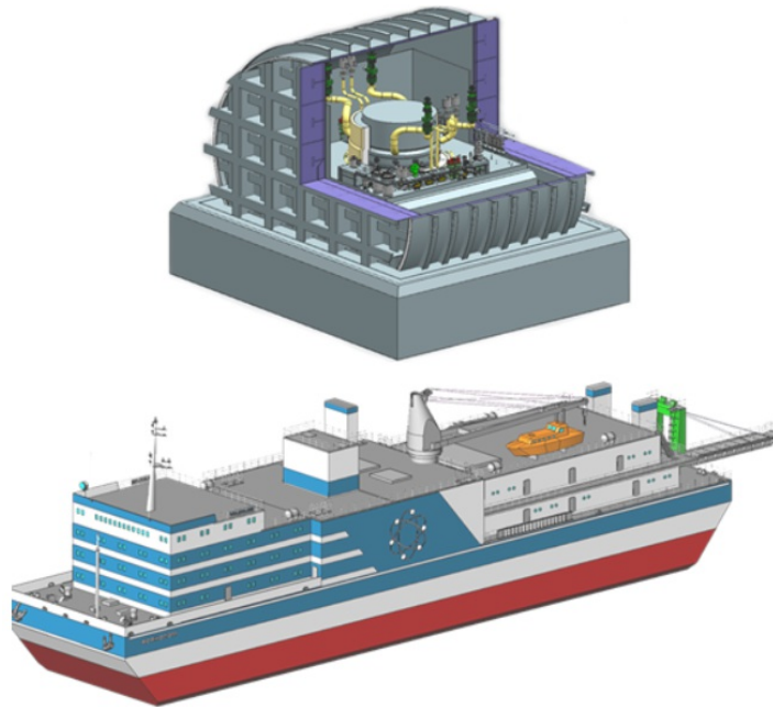
Figure 2. FPU and the reactor
