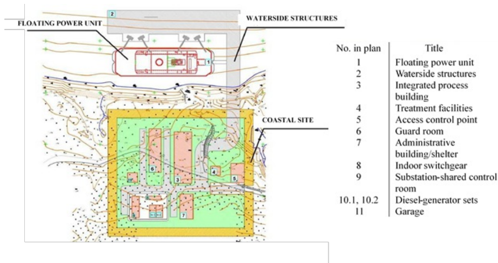
Figure 3. Plant layout
