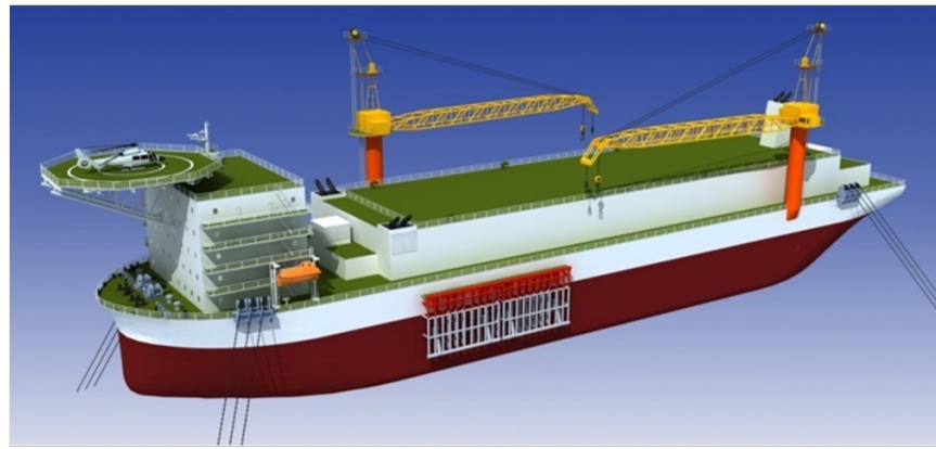
Figure 1. ACP100S design concept
