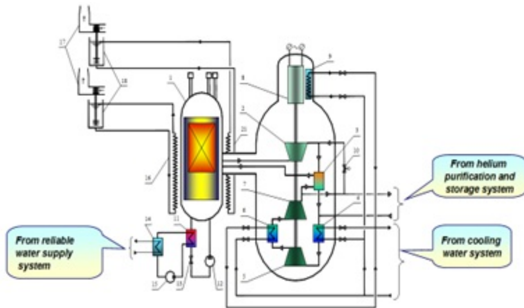
Figure 3. Power conversion system flow diagram
