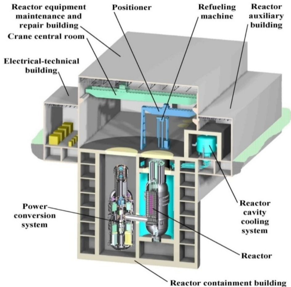
Figure 2. Plant layout
