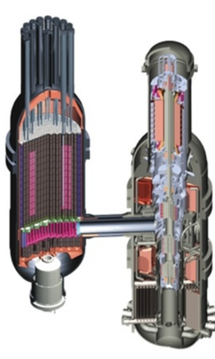
Figure 1. GT-MHR design concept
