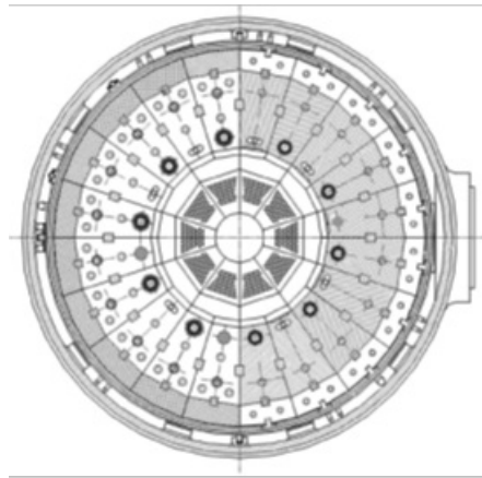
Figure 3. Reactor
