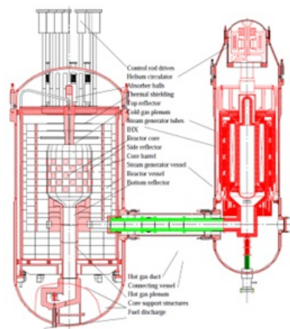
Figure 1. HTR-10 Concept design
