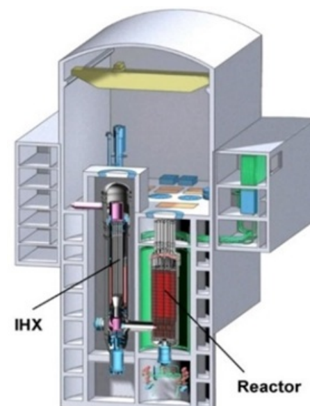
Figure 6. MHR-100 OR
