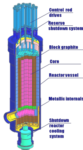
Figure 4. Reactor unit
