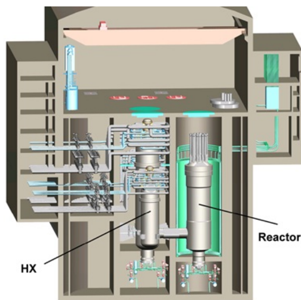
Figure 3. MHR-100 SMR
