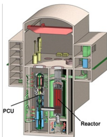
Figure 1. MHR-100 design concept
