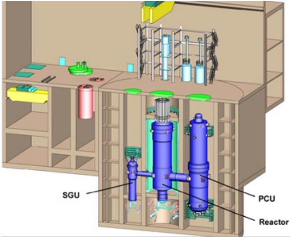
Figure 2. MHR-100 SE
