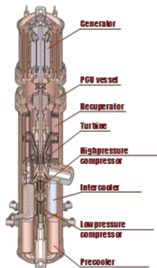
Figure 5. Power conversion unit
