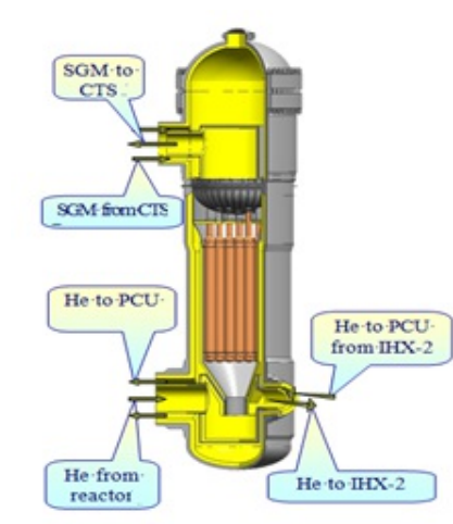
Figure 3. High temperature heat exchanger section
