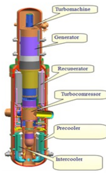
Figure 2. Power conversion unit
