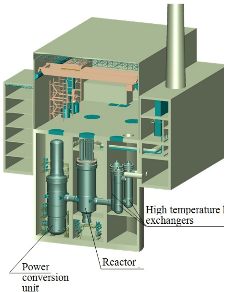
Figure 1. MHR-T design concept.
