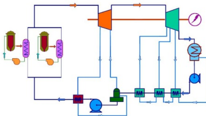
Fig. 1 - Simplified Schematic Diagram of the HTR-PM Demonstration Power Plant
