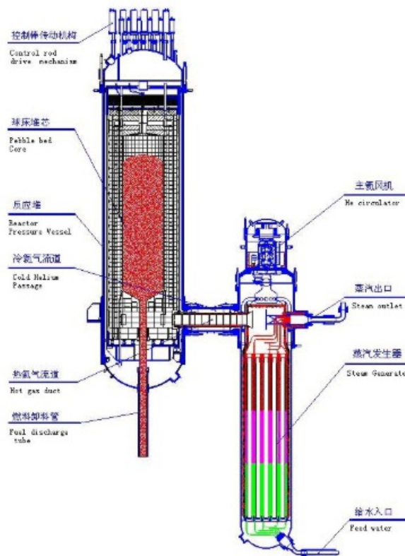
Fig. 3 - HTR-PM primary loop
