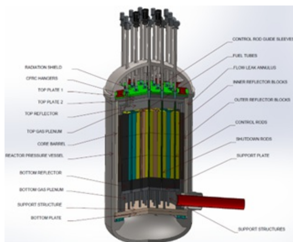
Figure 2. Reactor core
