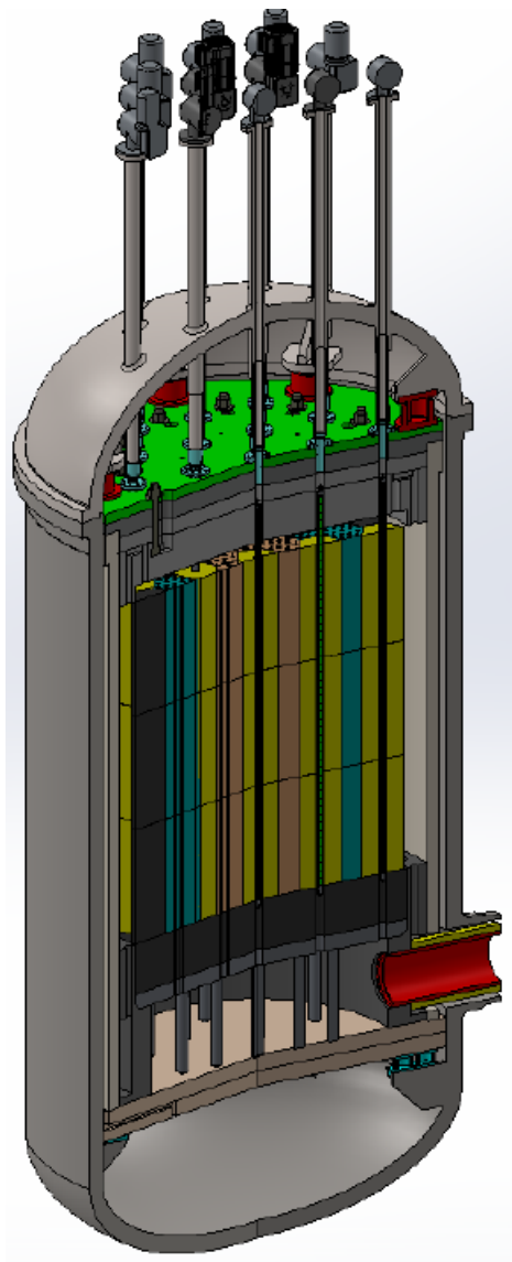
Figure 1. Design concept of AMR
