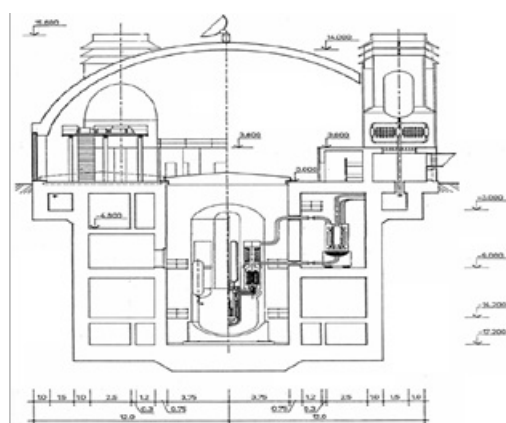
Figure 2. Reactor building
