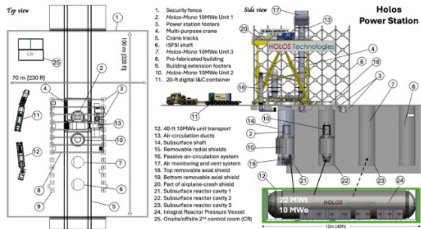
Figure 2. Plant layout
