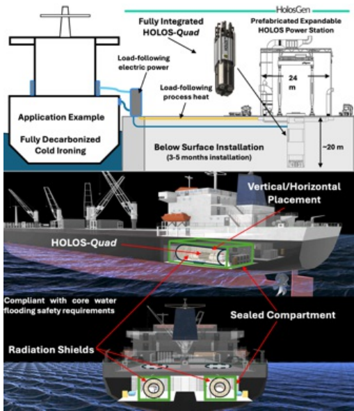
Figure 2. Layout and installation
