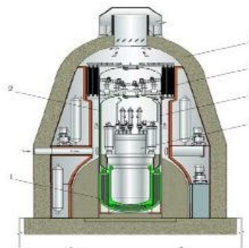
Figure 4. Containment system
