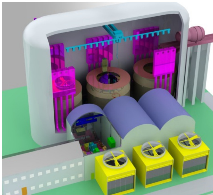
Figure 2. Cut-view of UNITHERM
