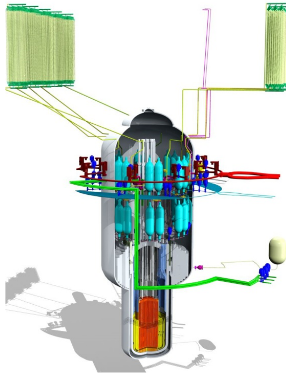
Figure 1. UNITHERM concept
