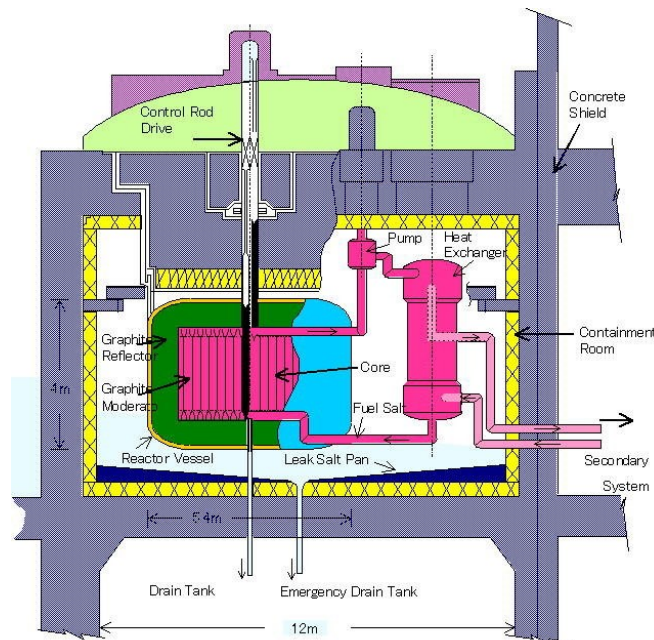
Figure 4. Vertical cross-section of MSR-FUJI
