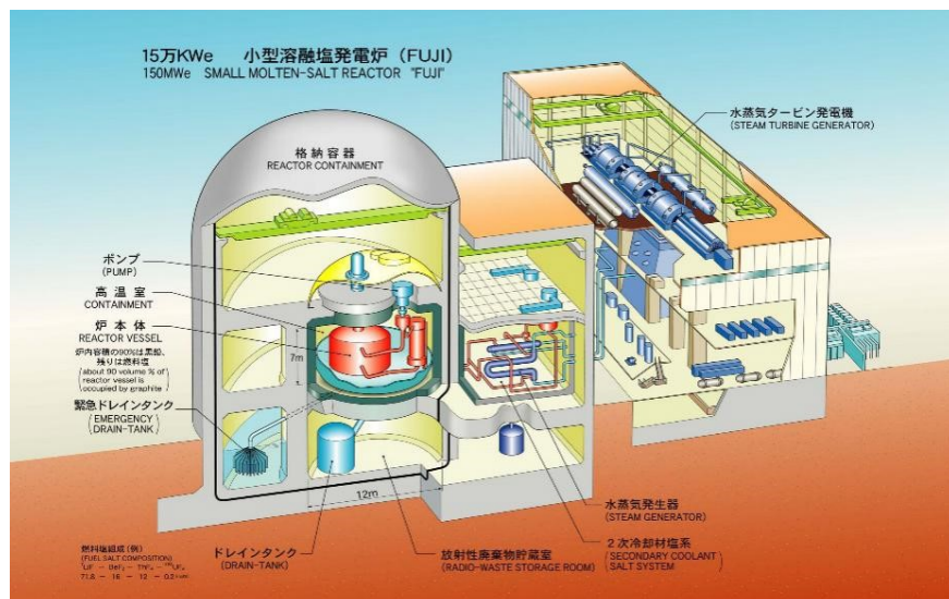
Figure 3. Bird's eye view of MSR-FUJI
