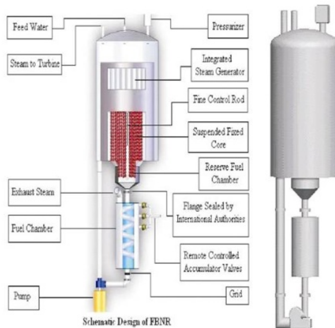
FIG. 4: Schematic design of FBNR
