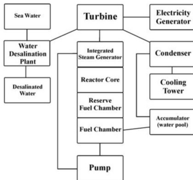
FIG. 2: Scheme of the Nuclear Power Plant
