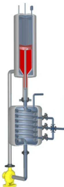
FIG. 5: Design of FBNR
