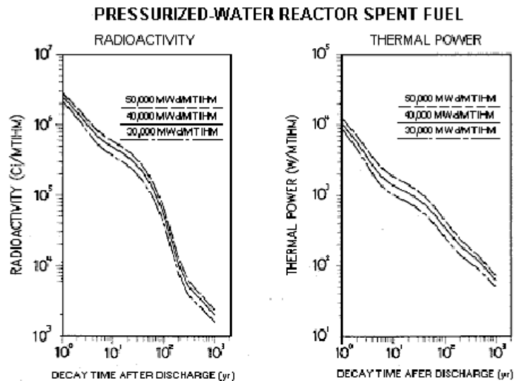
FIG. 7: Radioactivity and thermal power of the spent fuel as function of time
