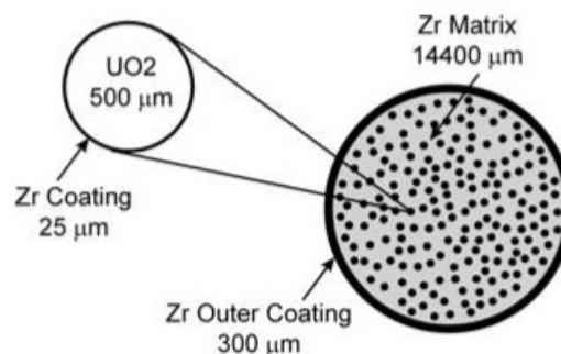
FIG 3: FBNR Fuel Element
