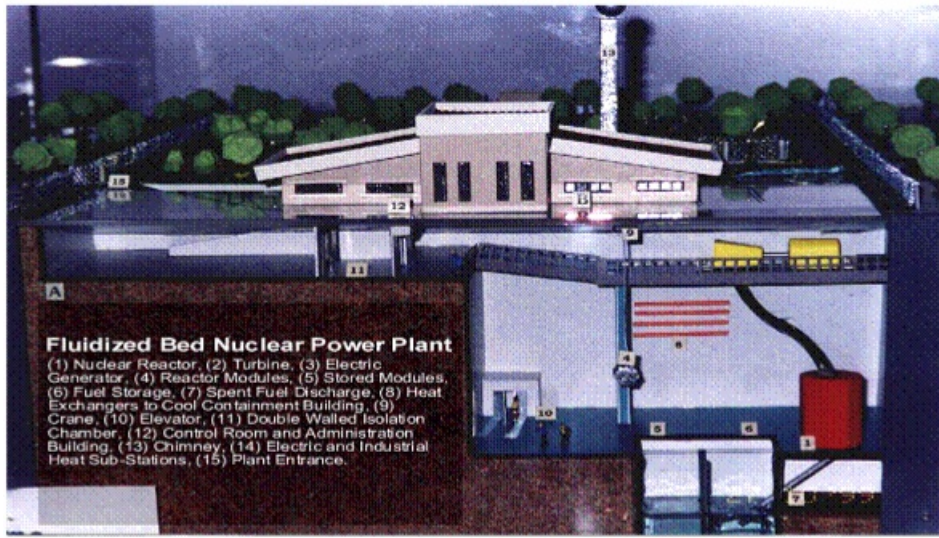
FIG. 1: FBNR Underground Containment Building
