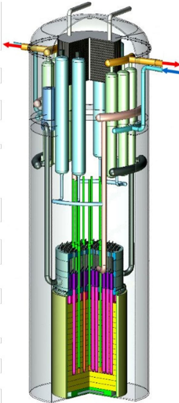
Figure 1. Representation of the STAR reactor.
