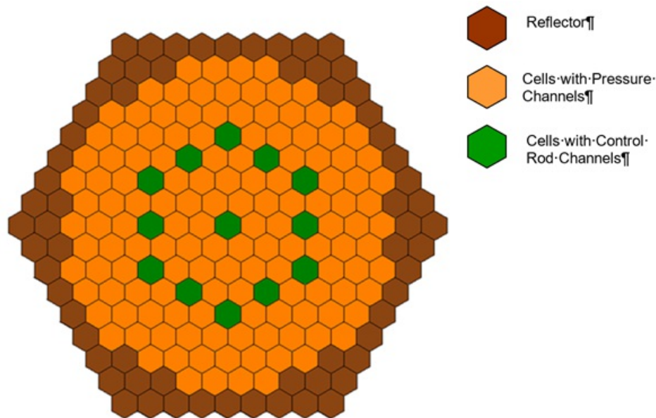
Figure 4. Reactor core layout.
