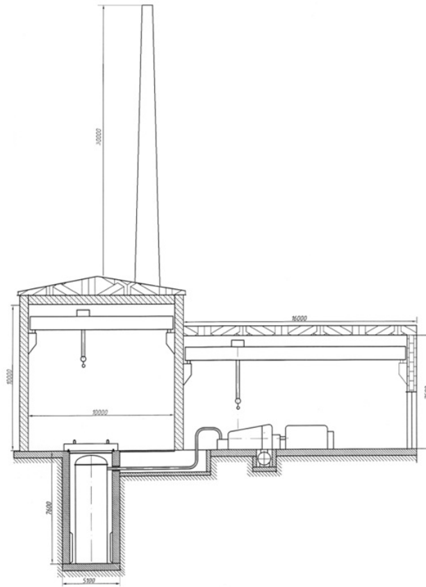
Figure 3. Example layout of a reactor building with an adjacent secondary island.
