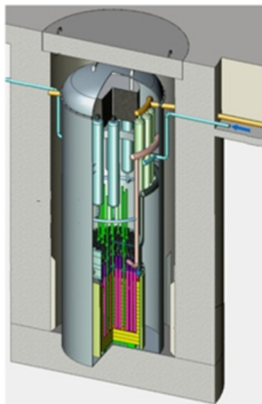
Figure 2. “STAR” module placement option inside an underground reactor shaft.
