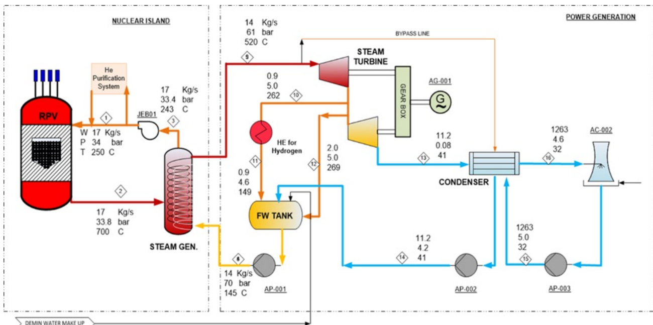
Figure 5. General process flow diagram of PeLUit-40.
