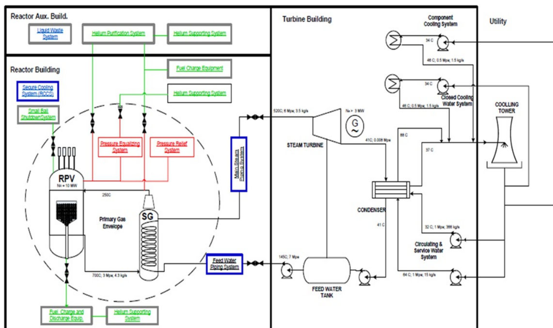
Figure 2. General schematic of building and system arrangement of PeLUit-40.
