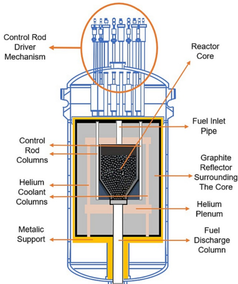
Figure 3. Main components of the RPV and its internals.
