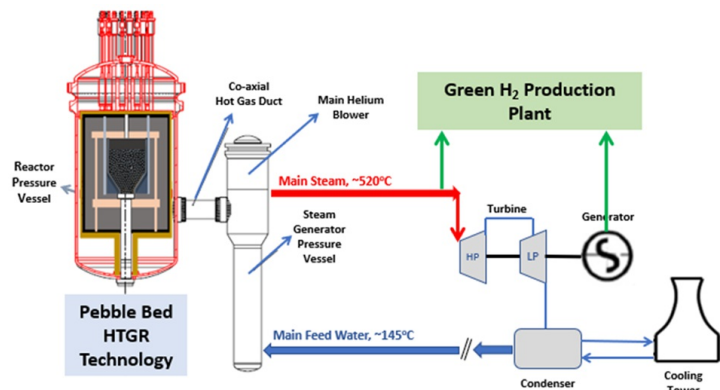
Figure 1. Schematic representation of a HTGR type reactor used in cogeneration mode for the production of hydrogen.
