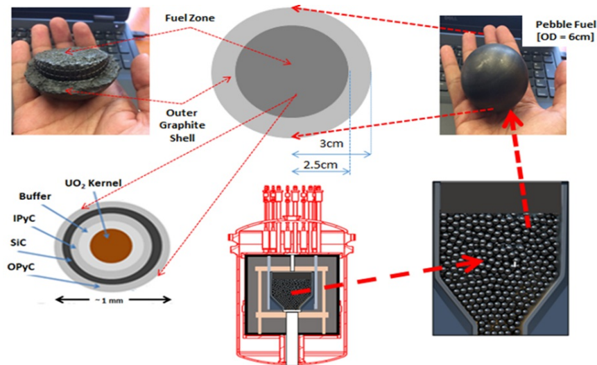
Figure 4. TRISO fuel.
