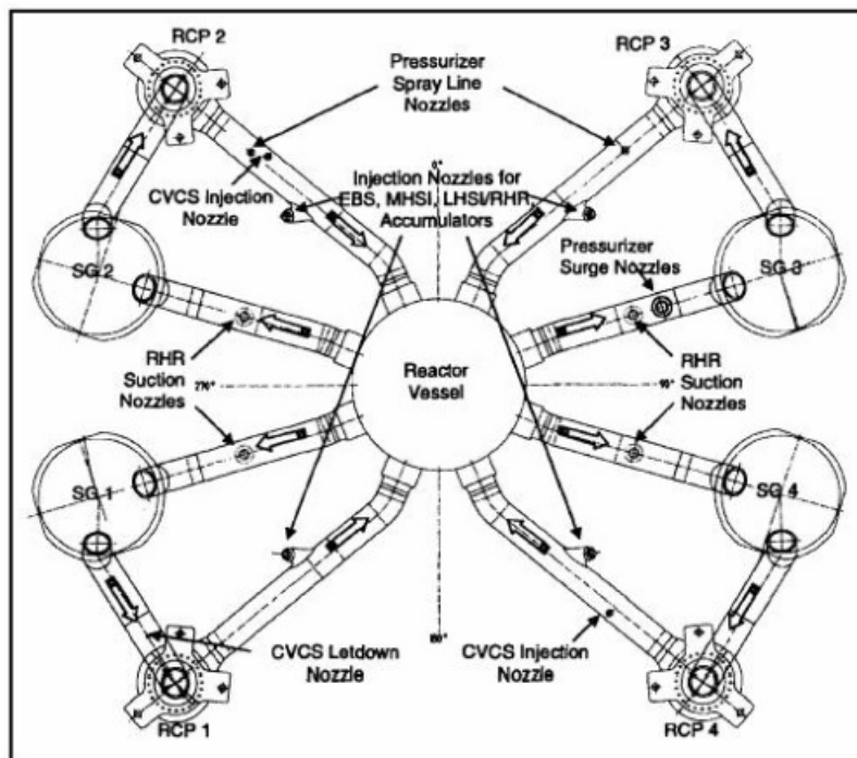
Figure 4 - RCS layout
