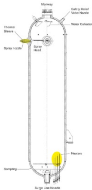
Figure 8 Pressurizer
