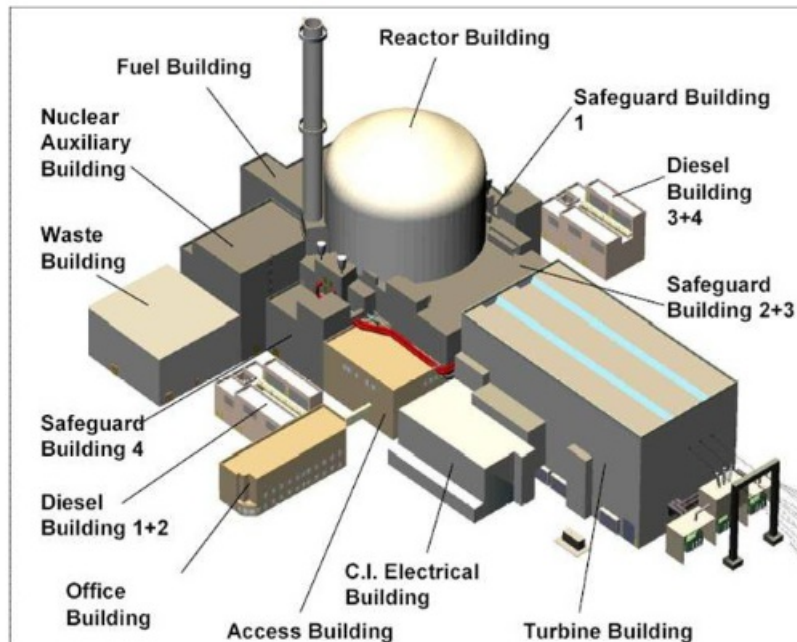
Figure 1 -. EPR™ 3D general view
