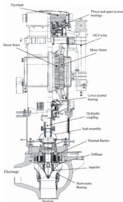
Figure 9 - Reactor coolant pump assembly
