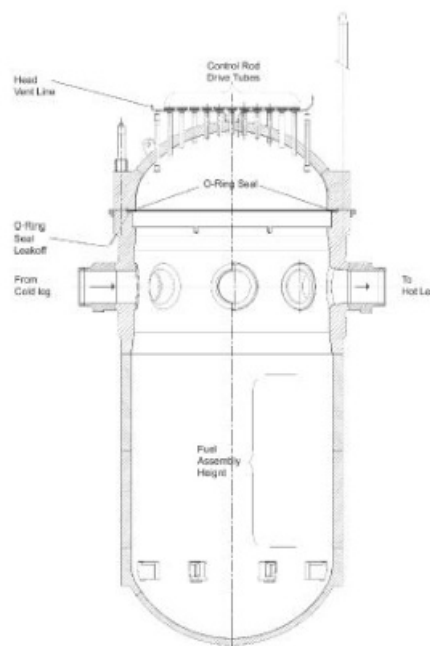
Figure 5 - Reactor pressure vessel
