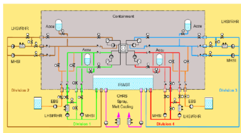
Figure 14 - Safety injection system
