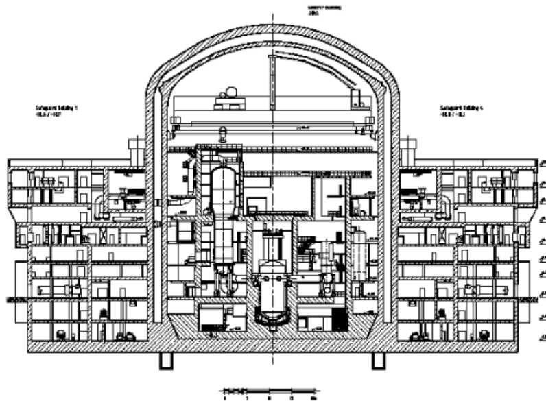
Figure 3 - Vertical cross section of the EPR™ reactor and safety buildings
