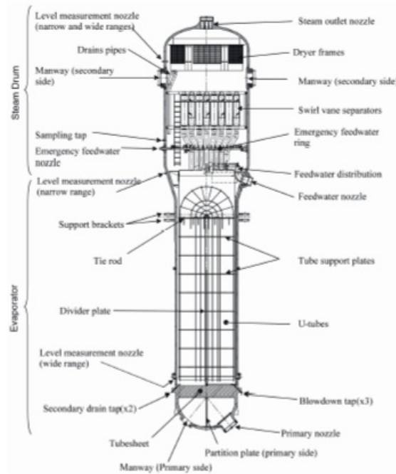
Figure 7 Steam generator
