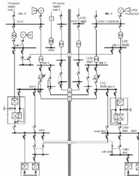
Figure 12 - Electrical single line diagram
