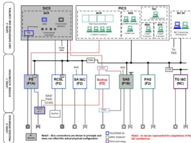
Figure 13 Overview of the standard EPR TM I&C architecture
