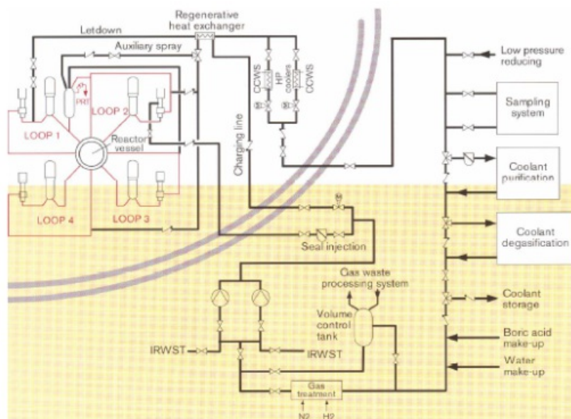
Figure 10 Chemical and Volume Control System
