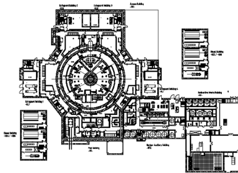
Figure 2 - EPR™ NI buildings – plan view at ± 0.00m
