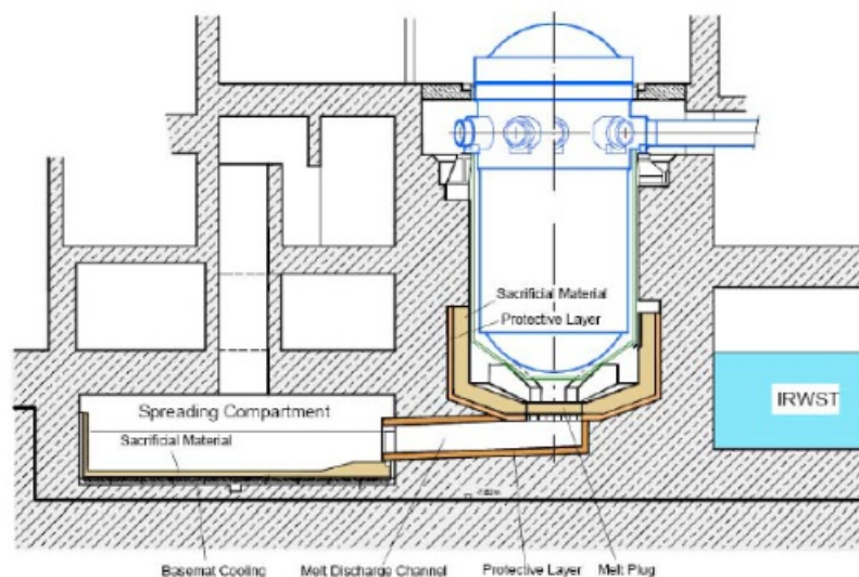
Figure 15 - Core melt retention system
